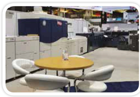
Xerox iGen™ 150 digital printing press working In-Line with a Bourg Sheet Feeder (BSF), a Bourg Peforating Rotating module (BPRF), a Bourg Binder BB3202 and a Three-Knife Trimmer CMT-330C
